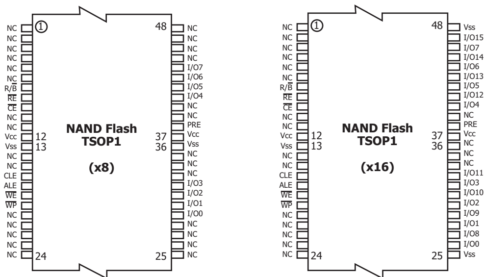
Figure 2. 48TSOP1 Contactations, x8 and x16 Device
