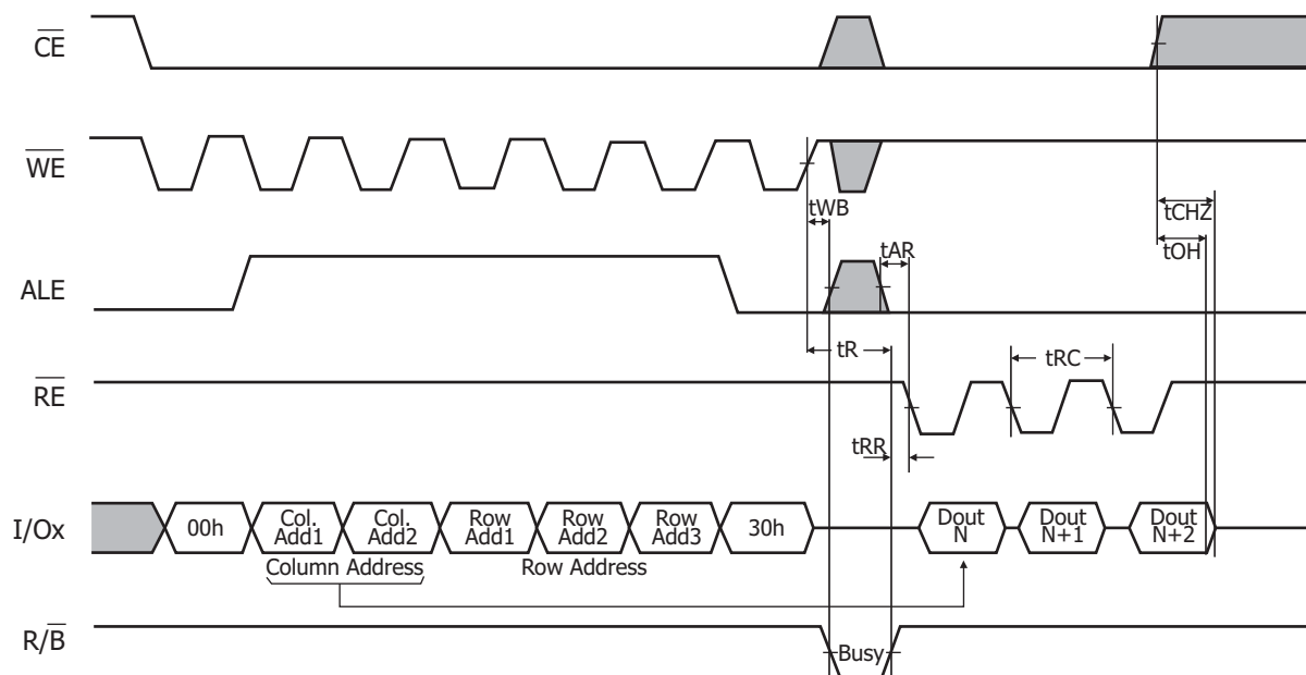
Figure 10: Read1 Operation intercepted by \overline{\text{CE}}\#
